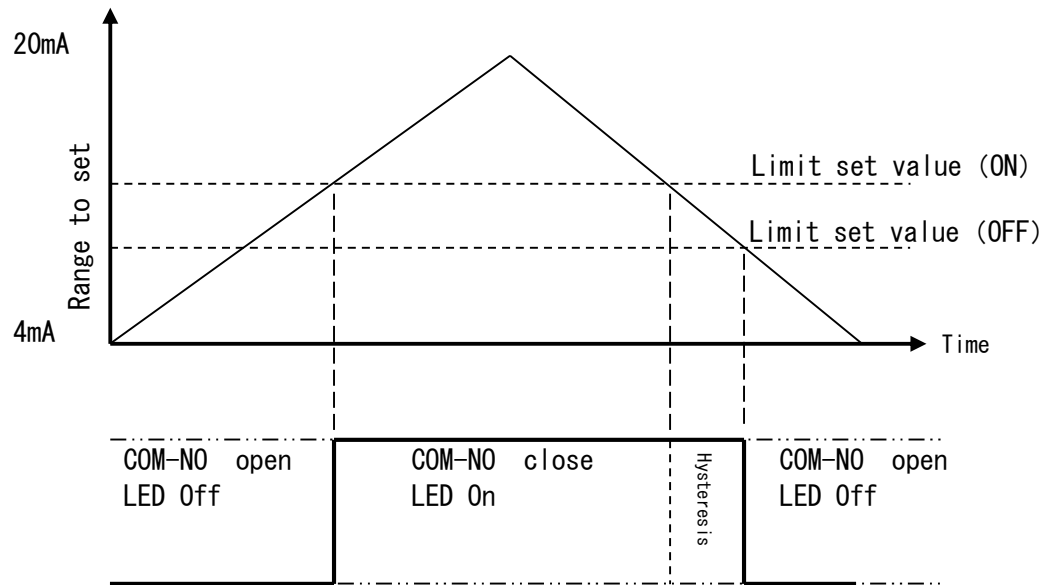
Fig.13. Operation chart (upper limit alarm)
