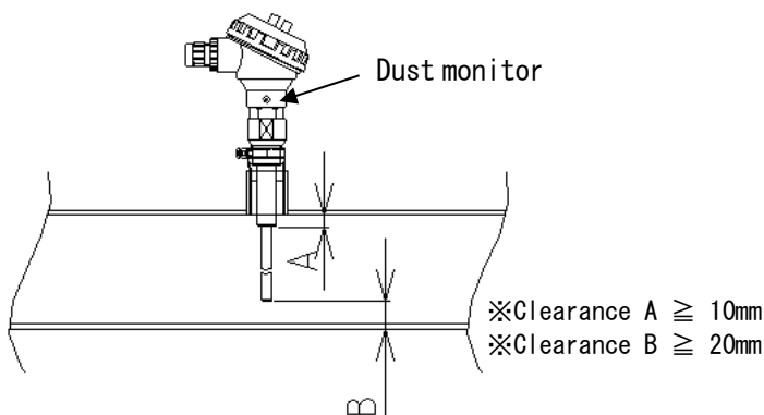
Fig. 5. Installation reference figure
