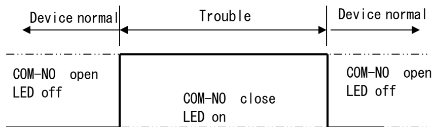
Fig.14. Operation chart (Trouble alarm)
