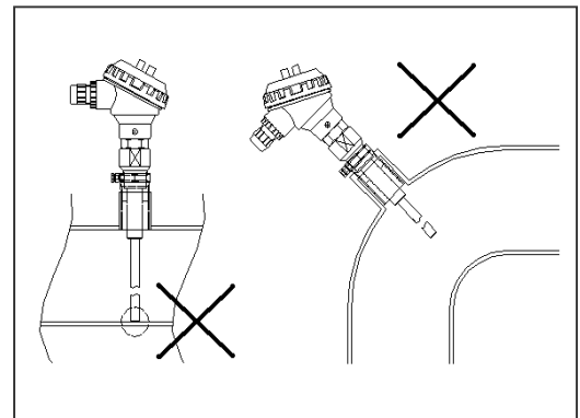
Fig. 4. Example) Installation not good
