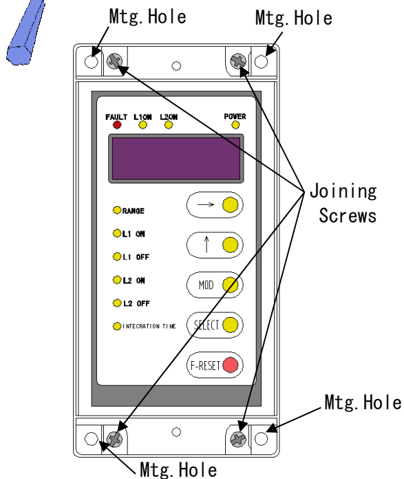
Fig. 7. Joining screws of terminal and main block part
