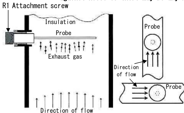
Fig. 3. Installation
