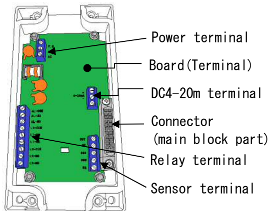
Fig. 8. Terminal part
